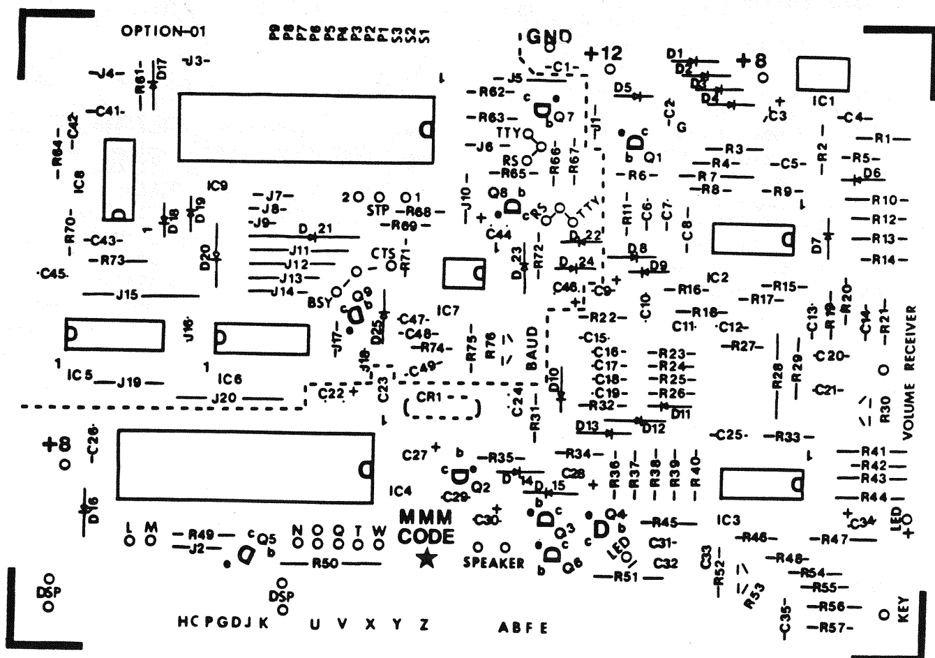
Legend Side - Main PC Board
