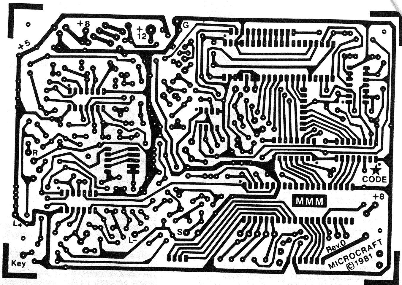
Foil Side - Main PC Board
